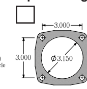
Symmetrical H1131
