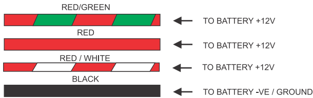
Figure 6 - Battery Wiring
