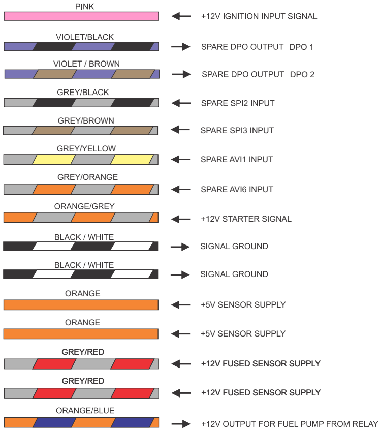
Figure 5 - Cabin Harness Wiring
