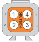
DTM-4 Connector
