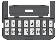
Tyco 16 Position Auxiliary Connector
